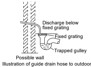
Illustration of guide drain hose to outdoor
